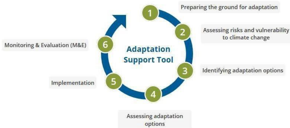
Figure 4-2. Adaptation support tool. Source: Climate-ADAPT.
