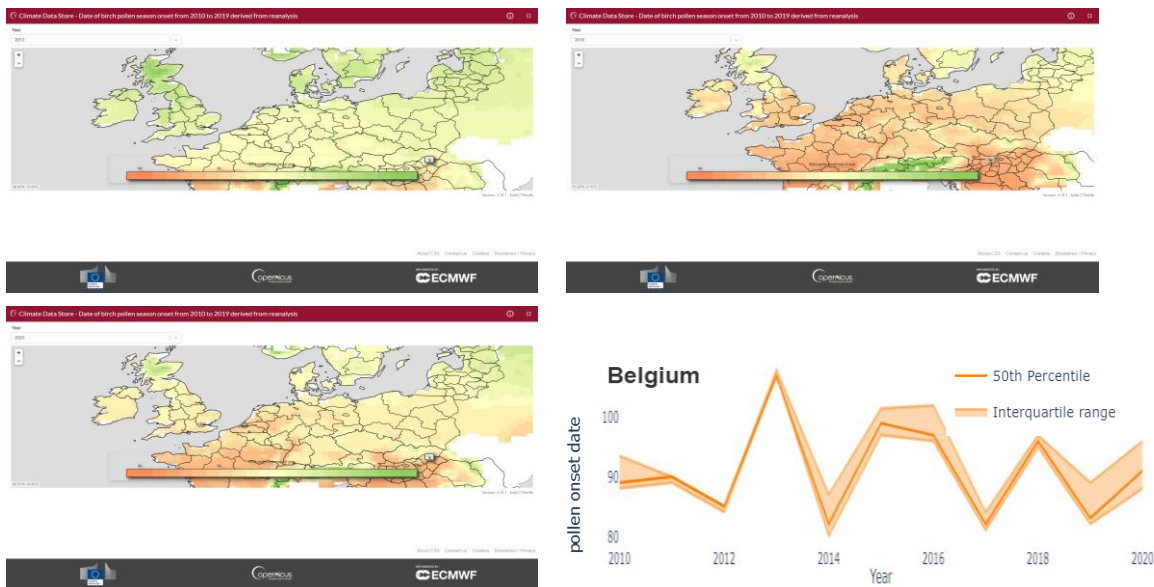
Figure 5-16. Yearly variation in onset (day of the year) of the birch pollen season based on ERA5 reanalysis data. Maps highlight onset over Europe in 2013, 2019 and 2020 (orange colours indicating earlier onset than green colours) and the graph shows the interannual variation in average onset (+ interquartile range) for the Belgian territory. Source: Copernicus Climate Data Store 1 .
